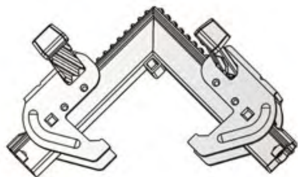
KRL Clamp Weight: 7.1kg
