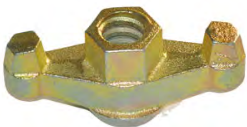
Size:W100xH45mm Weight:0.39kg Type:DW15
